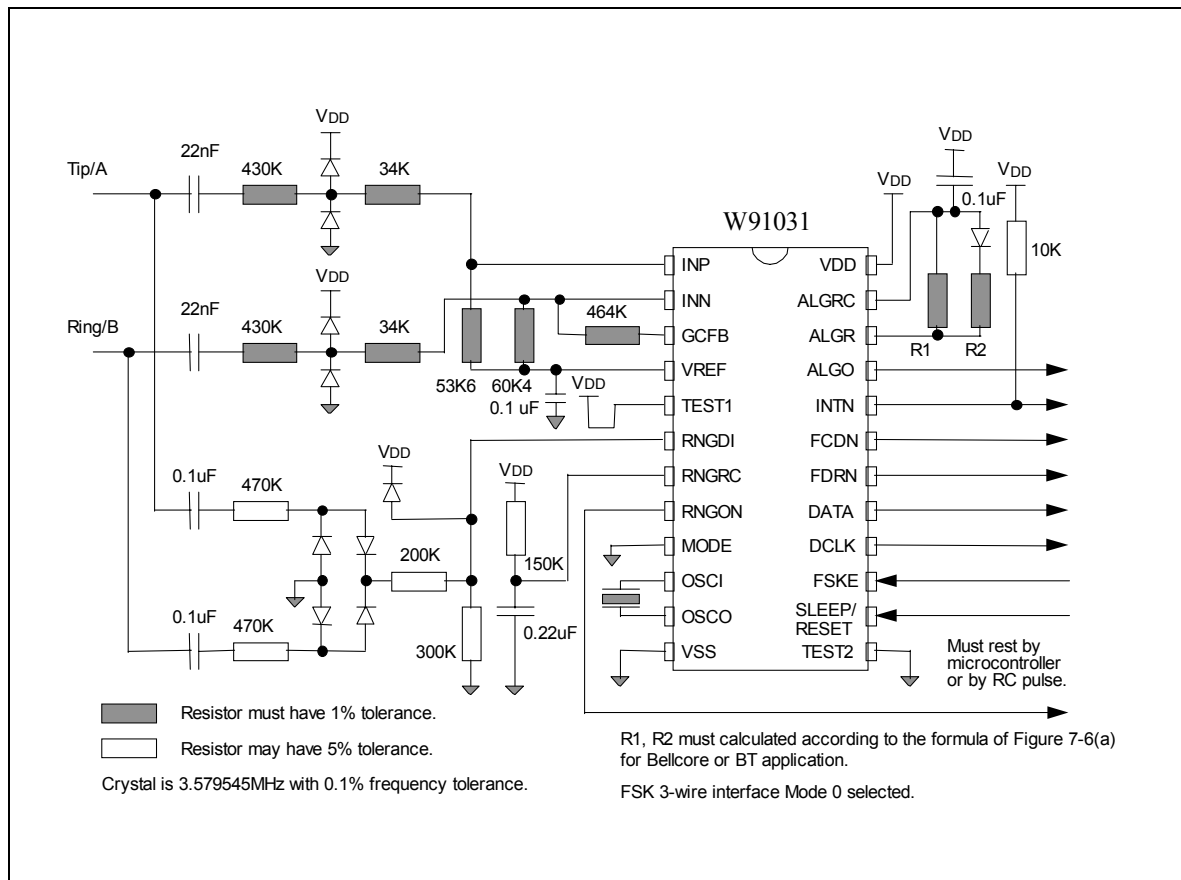
Figure 9-1. Application Circuit.
